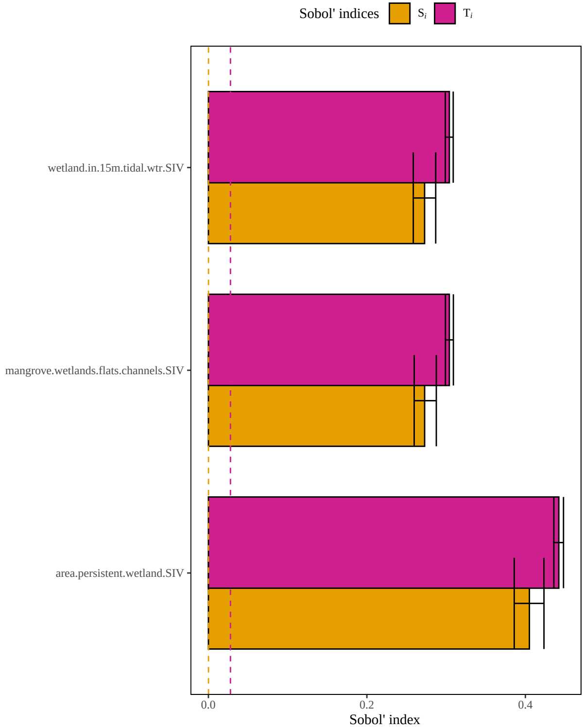
Figure 5. Results of a sensitivity analysis for the clapperrail model based on a geometric mean structure. Dashed lines represent baseline numerical approximation error for S_i and T_i ( i.e. , dummy variables).
