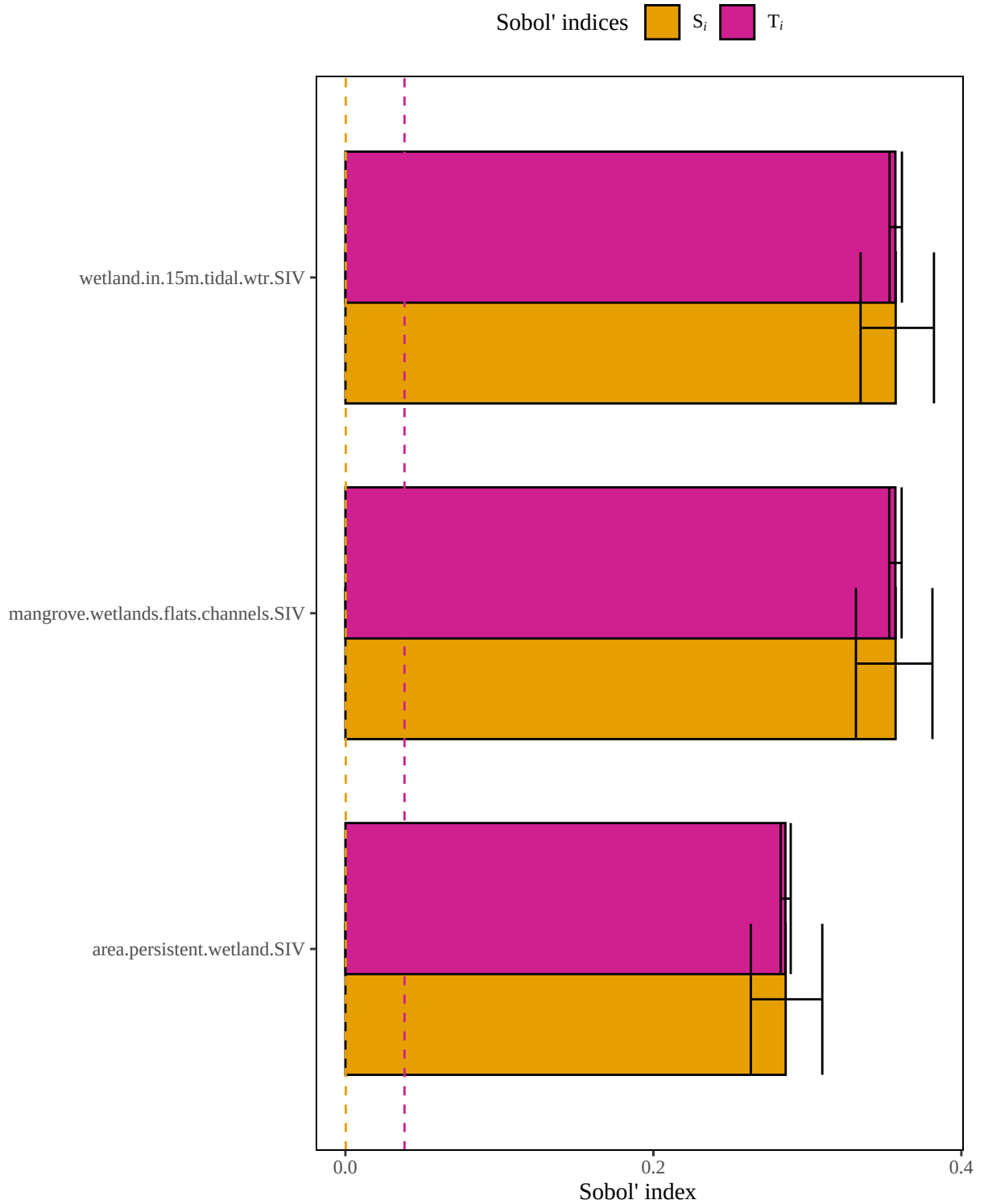
Figure 4. Results of a sensitivity analysis for the clapperrail model based on an arithmetic mean structure. Dashed lines represent baseline numerical approximation error for S_i and T_i ( i.e. , dummy variables).
